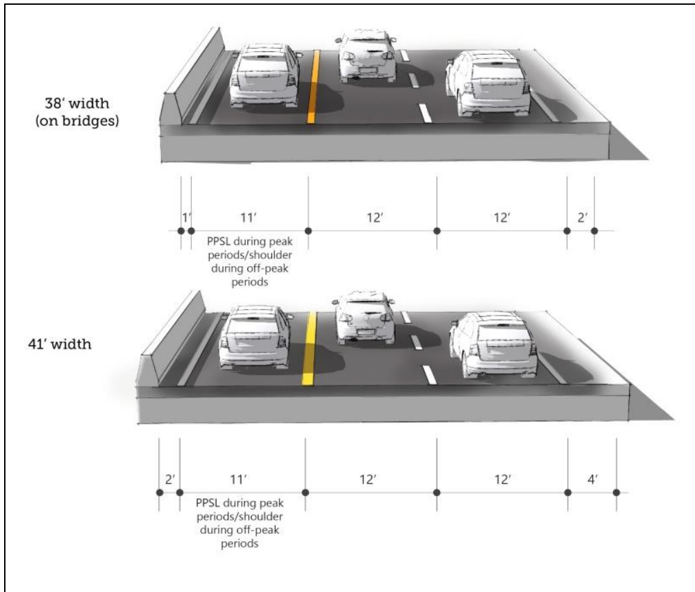
Figure 3. WB PPSL Proposed Action Typical Cross Sections
